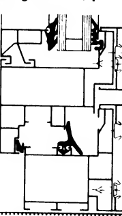
⑦ Plastic window with aluminium facing frame (up to 42 dB)
